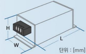
W3 / W3COM 441(W)×88(H)×390/430(L) (W) : 약 5mm 축소값 반영됨 (2021.08)
