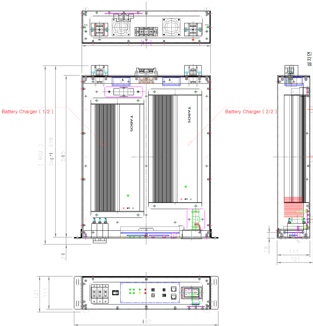
( Internal Structural Drawing )
