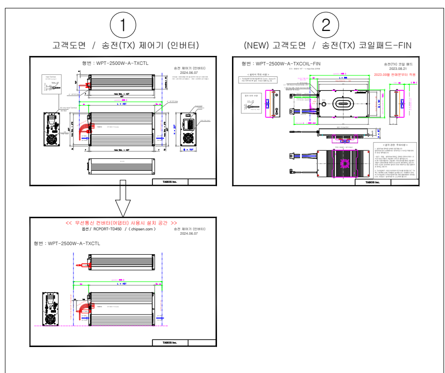
송전부(TX)
