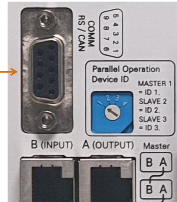
D_SUB 9핀 / Female (암)
